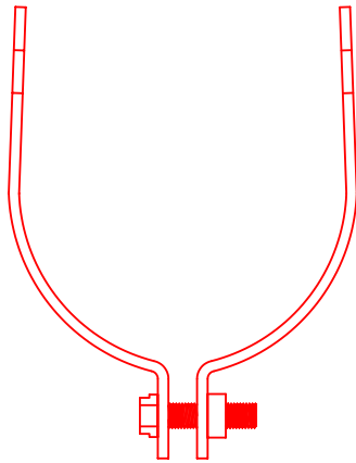
3-1/8" 2 Piece Metal Clamp (2 per Cell) PN 310023
