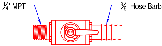
PVC Shut Off Valve PN 360006
