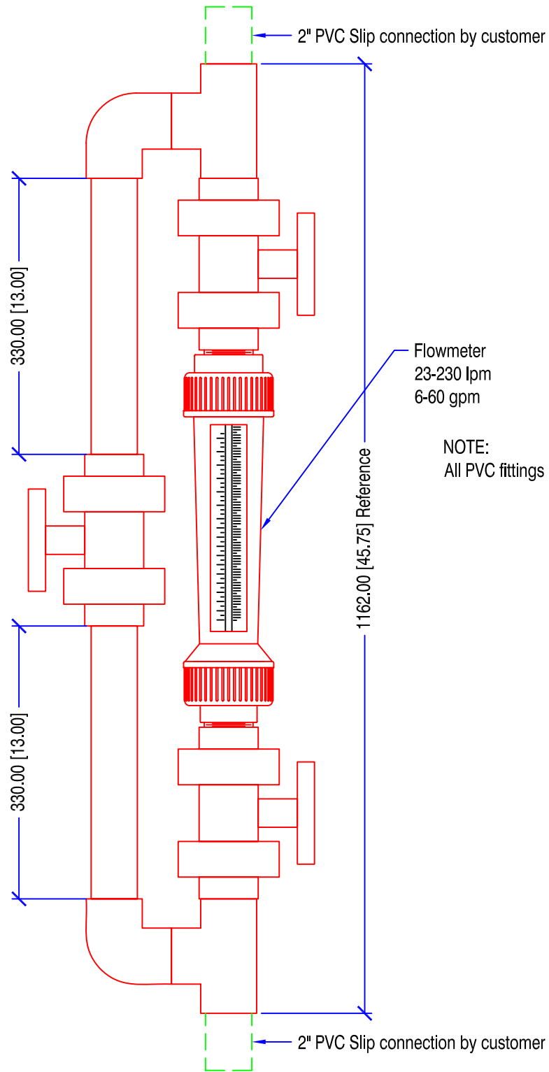
Side View
