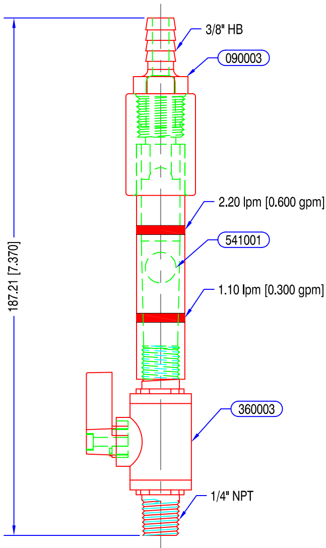
Side View
