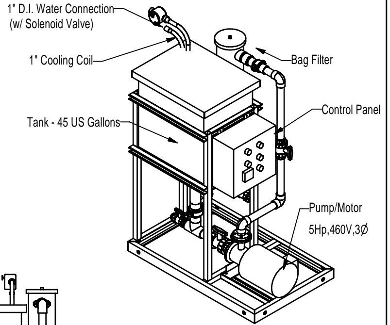
Isometric
